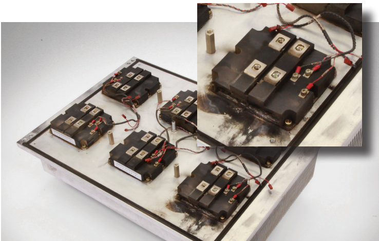
A blown Xantrex Matrix Inverter from a GE 1.5MW S Series wind turbine.
